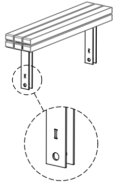
4003C - Casting
