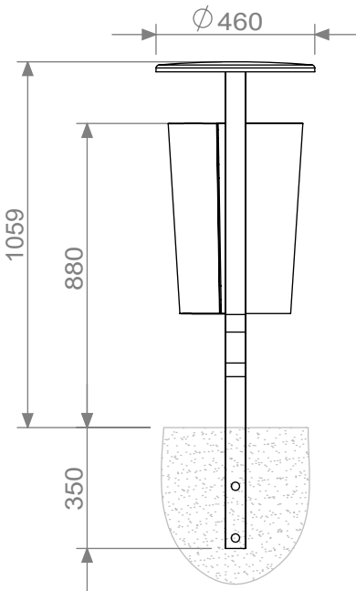
Type C - Casting in the ground
